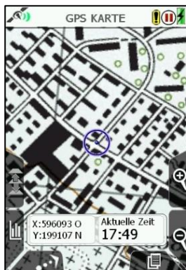
Zu Positionsinfo
