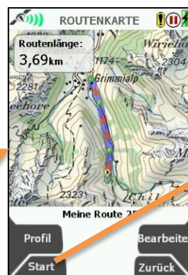
Routenkarte
